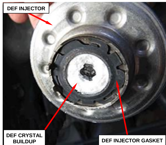
Figure 17 – DEF Injector Gasket
