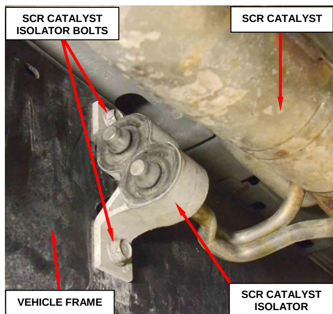
Figure 29 – SCR Catalyst Isolator
