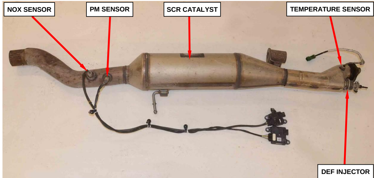
Figure 15 – Selective Catalytic Reduction (SCR) Catalyst Assembly
