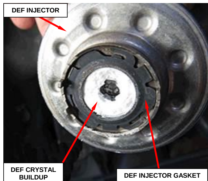
Figure 34 – DEF Injector Gasket
