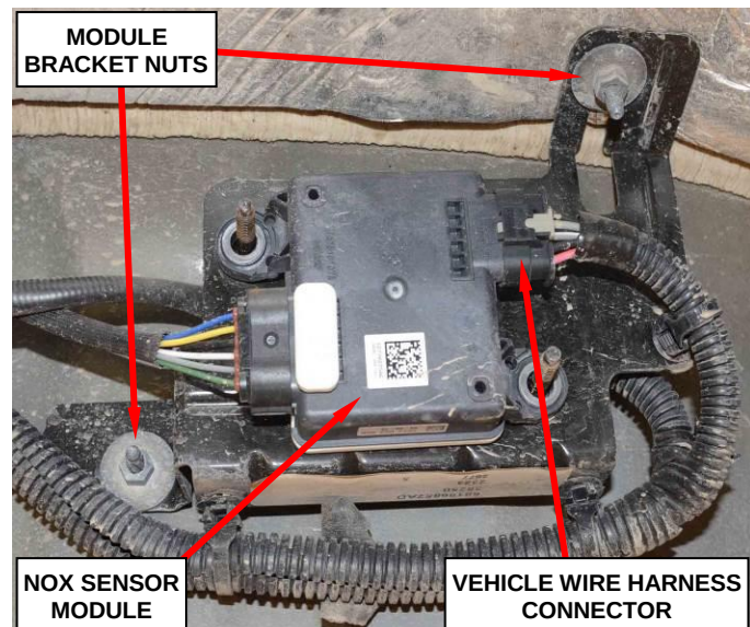
Figure 9 – NOx Sensor Module
